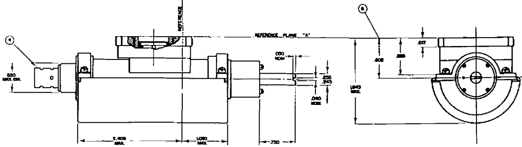
OUTLINE DRAWING ELECTRON TUBE OK 797/RK 7521
