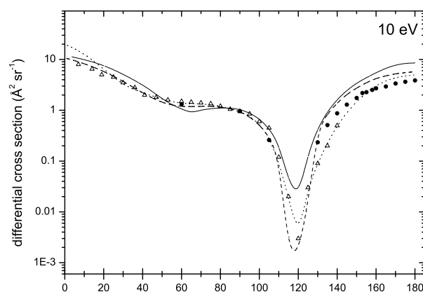
Fig. 2. Differential cross sections versus scattering angle. Solid line: current results, full circles: experimental results of Mielewska [14], empty triangles: experimental results of Furst et al. [15], dashed line: Pleniewicz et al. [16] (pseudopotential approach), dotted line: Syty and Sienkiewicz [13] (CI-MCDF).
