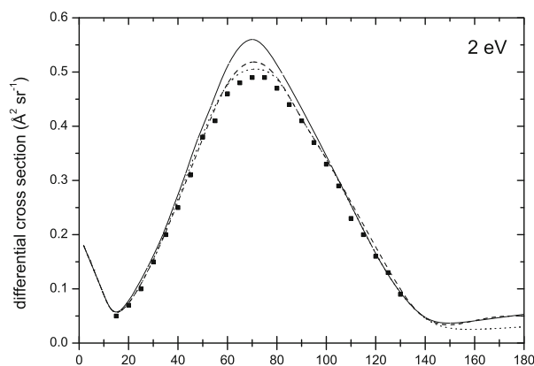
Fig. 1. Differential cross sections versus scattering angle. Solid line: current results, full squares: experimental results of Gibson et al. [11], dashed line: McEachran and Stauffer [12] (relativistic polarized-orbital method), dotted line: Syty and Sienkiewicz [13] (CI-MCDF).
