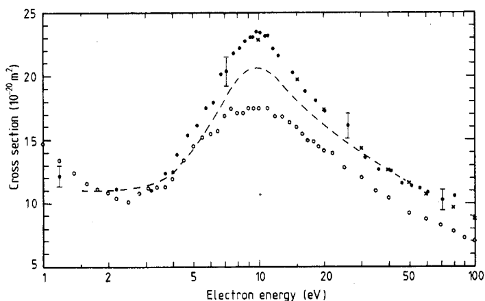
Figure 1. Total cross sections for electron-ammmonia scattering. Experiment: ●, present results, absolute; ---, Brüche (1929), absolute; ○, Sueoka et al (1987), normalised. Theory: +, Jain (1988). The error bars correspond to the overall experimental uncertainties at some selected points.
