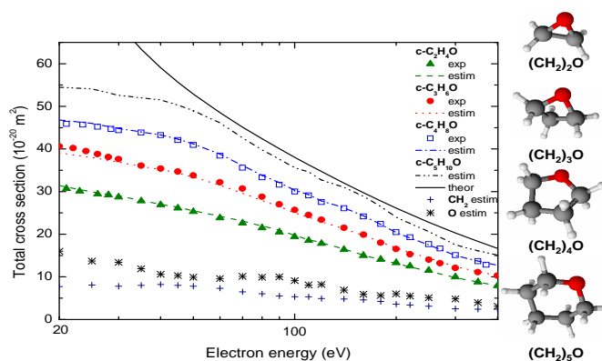
Figure 2: Comparison of the experimental or calculated TCSs with those estimated from group additivity rule for e^- -scattering by (\text{CH}_2)_n\text{O} , n=2-5 . Experimental data: c\text{-}(\text{CH}_2)_2\text{O} (Szymtkowski et al. 2008a), c\text{-}(\text{CH}_2)_3\text{O} (Szymtkowski et al. 2008b) and c\text{-}(\text{CH}_2)_4\text{O} (Możejko et al. 2006). Theoretical TCS for c\text{-}(\text{CH}_2)_5\text{O} is the sum of elastic and ionization cross sections. Molecule pictographs are included.
